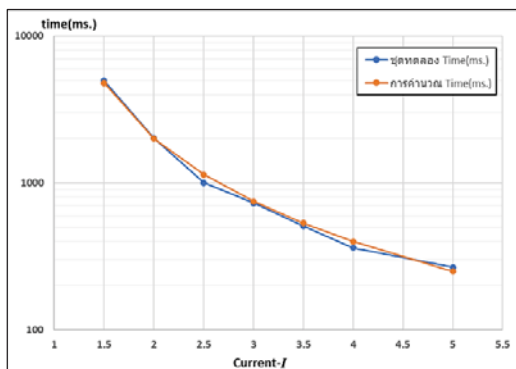
(c) Extremely Inverse
